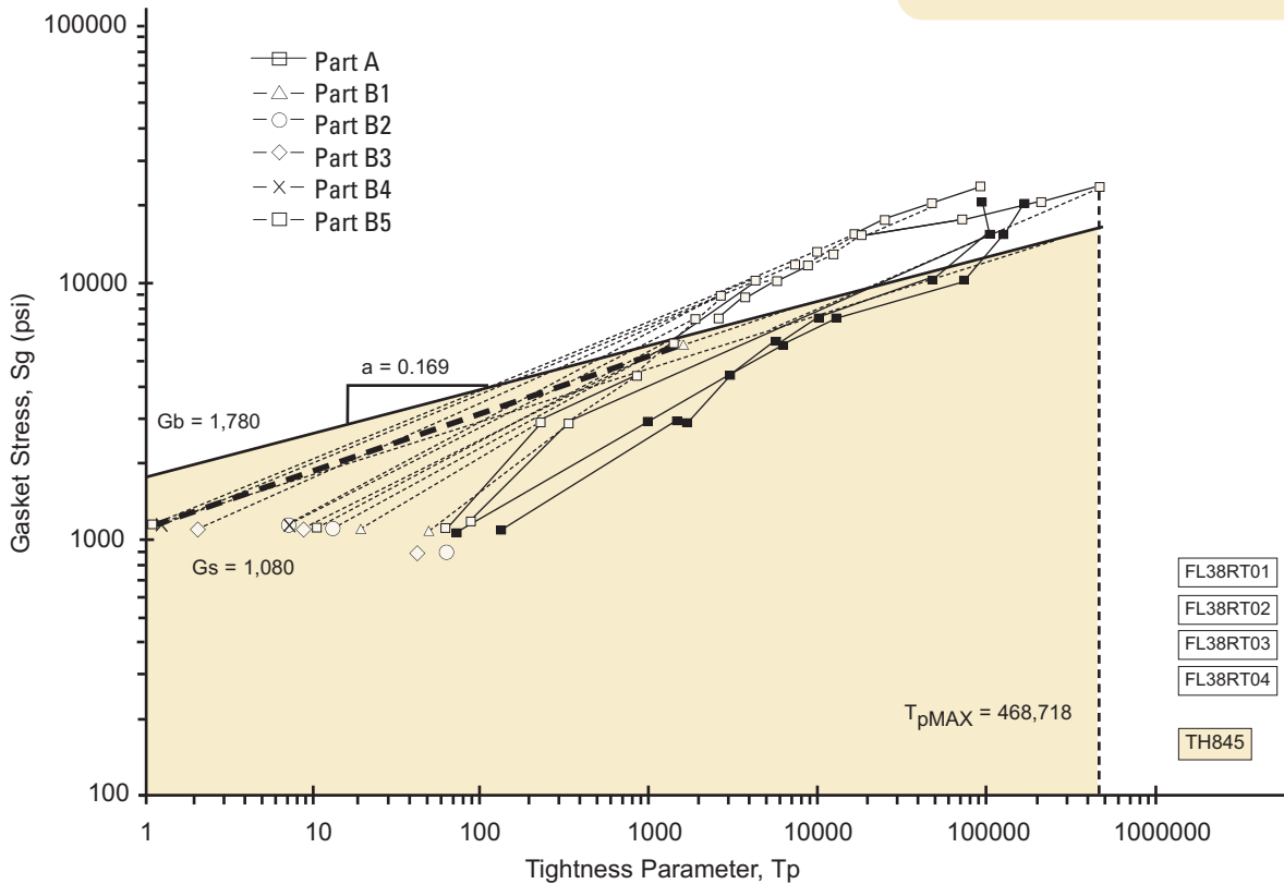
CRITICAL SERVICE SERIES Thermiculite® 845, high temperature facing for Flexpro (Kammprofile) gaskets.
